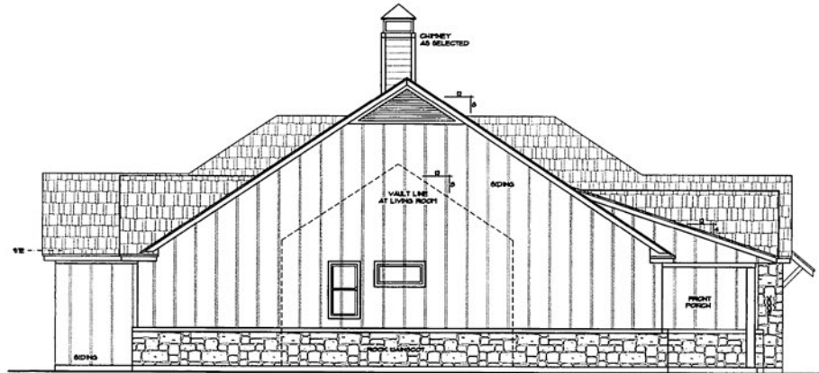
LEFT ELEVATION
